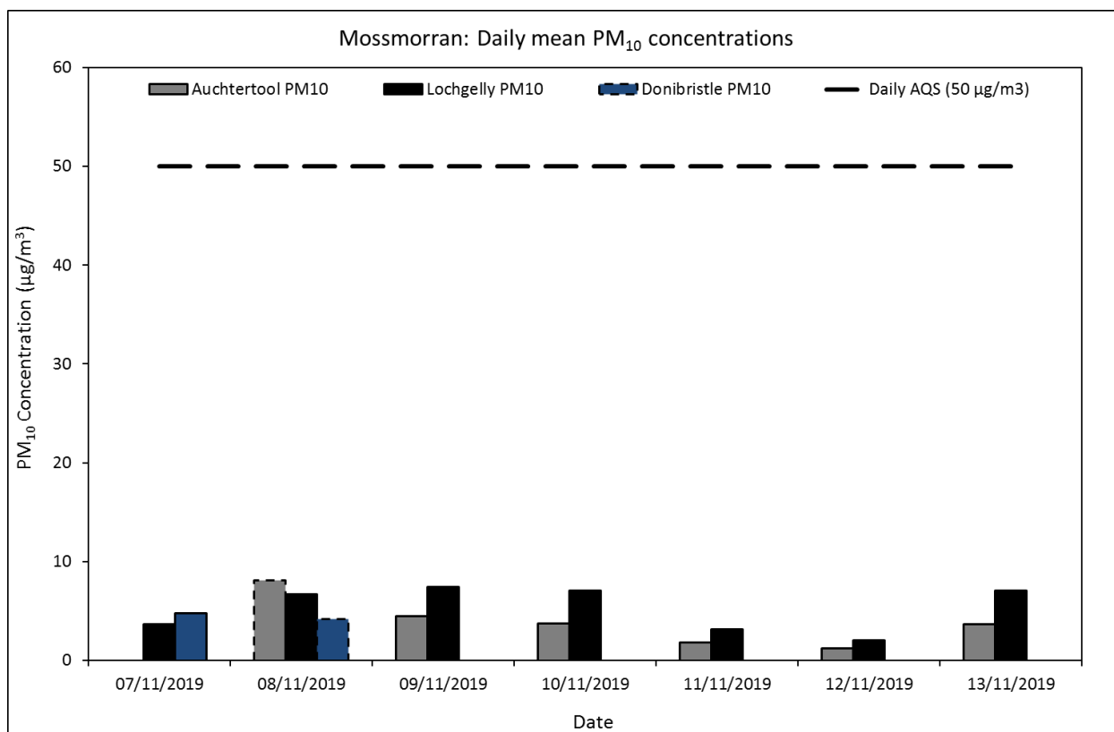
Figure 4: Daily rolling means for PM 10 at Lochgelly, Auchtertool and Donibristle. Dotted lines represent mean values based on less than 24 hours of data collection.
