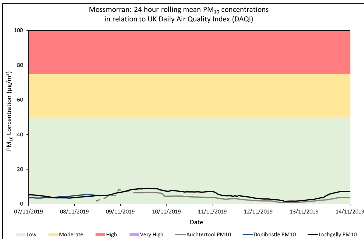
Figure 2: 24 hour rolling means for PM 10 at Lochgelly, Auchtertool and Donibristle. Dotted lines represent mean values based on less than 24 hours of data collection.
