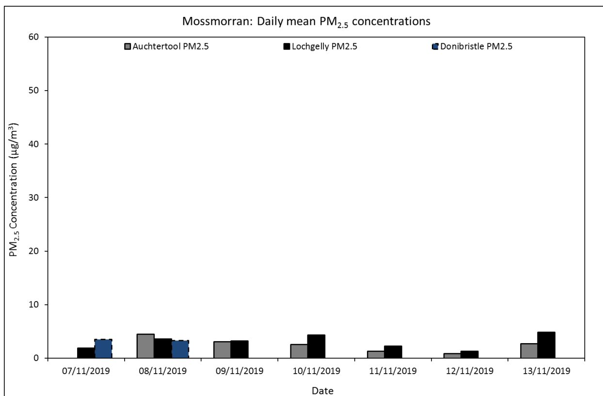
Figure 5: Daily rolling means for PM 2.5 at Lochgelly, Auchtertool and Donibristle. Dotted lines represent mean values based on less than 24 hours of data collection.
