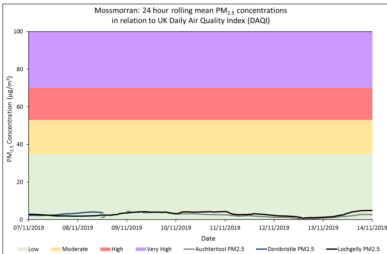
Figure 3: 24 hour rolling means for PM 2.5 at Lochgelly, Auchtertool and Donibristle. Dotted lines represent mean values based on less than 24 hours of data collection.
