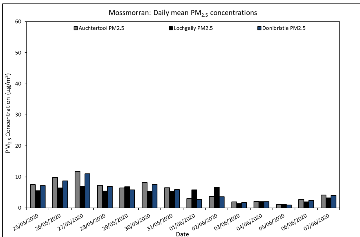
Figure 4: Daily means for PM 2.5 at Lochgelly, Aughtertool and Donibristle. Dotted lines represent mean values based on less than 24 hours of data collection.
