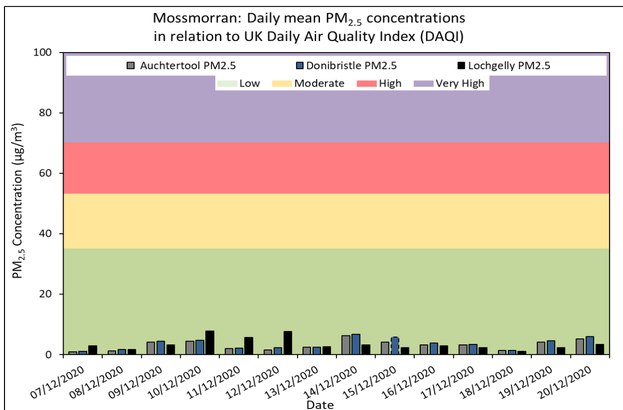
Figure 4: Daily means for PM 2.5 at Lochgelly, Auchtertool and Donibristle. Dotted lines represent mean values based on less than 24 hours of data collection.
