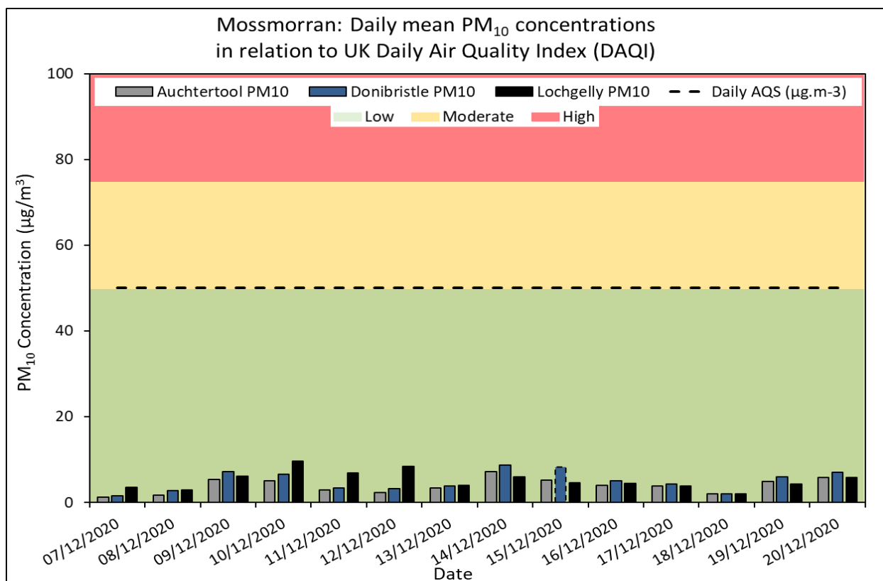
Figure 3: Daily means for PM 10 at Lochgelly, Auchtertool and Donibristle. Dotted lines represent mean values based on less than 24 hours of data collection.
