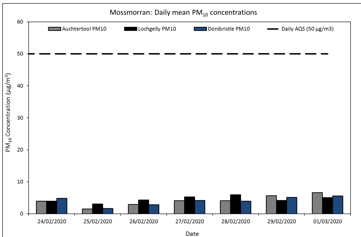
Figure 3: Daily rolling means for PM 10 at Lochgelly, Auchtertool and Donibristle. Dotted lines represent mean values based on less than 24 hours of data collection.
