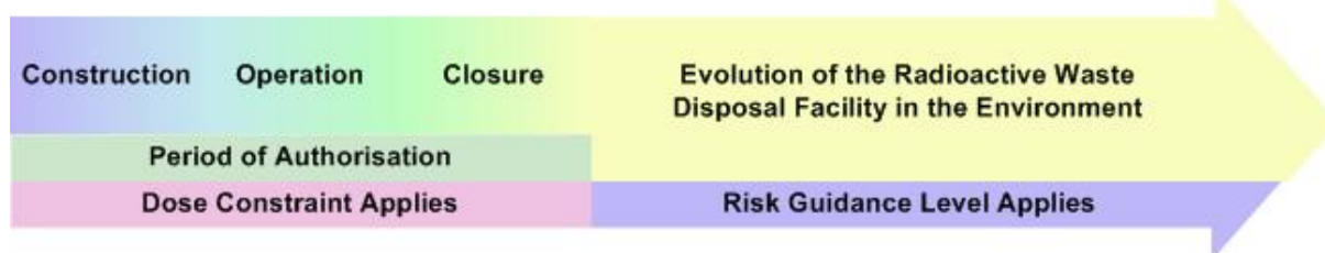
Figure 6.1 Periods of applicability for the dose constraint and the risk guidance level.
