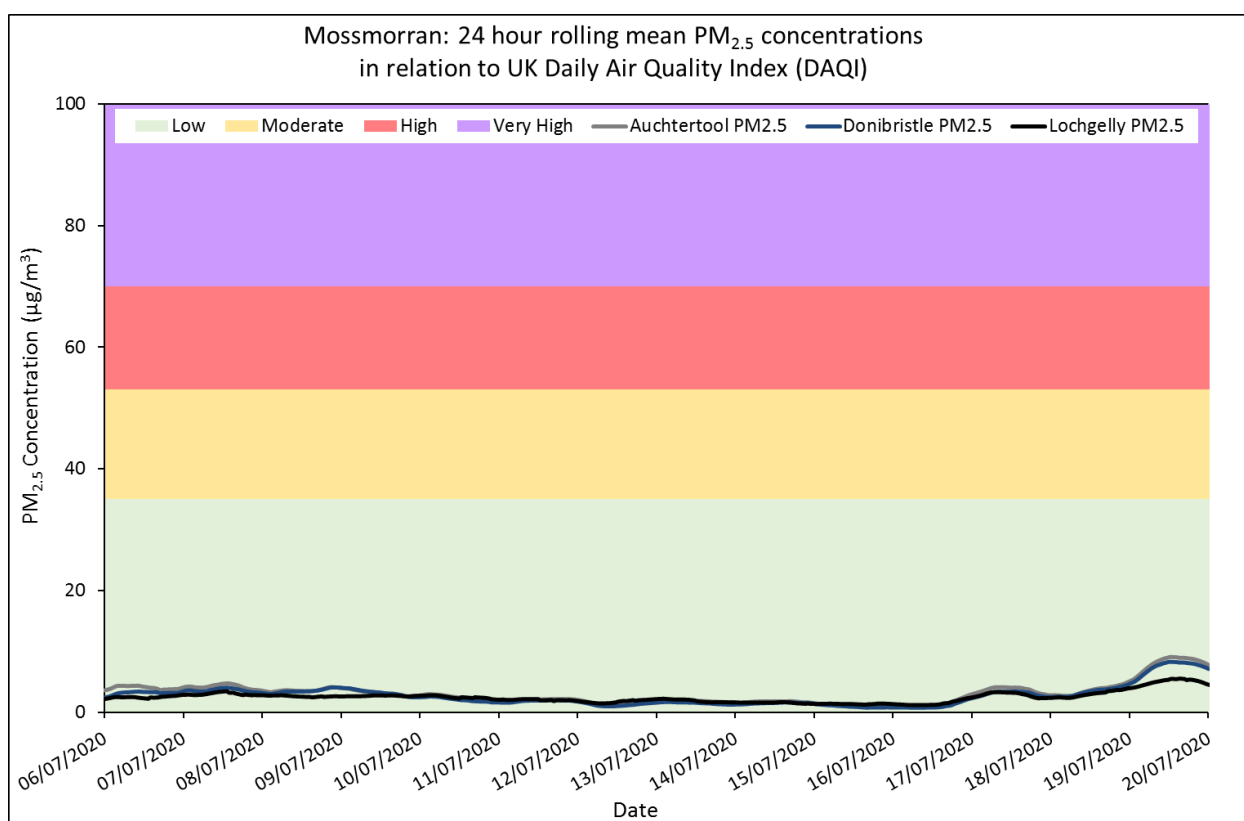
Figure 2: 24 hour rolling means for PM 2.5 at Lochgelly, Aughtertool and Donibristle. Dotted lines represent mean values based on less than 24 hours of data collection.
