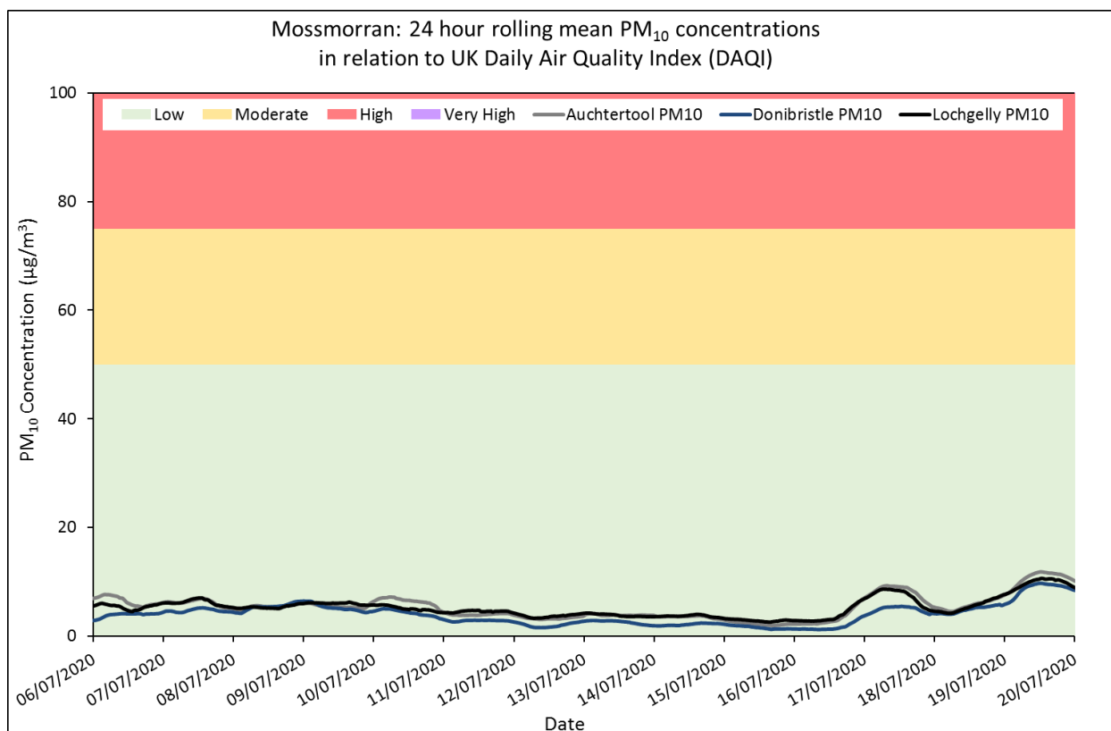
Figure 1: 24 hour rolling means for PM 10 at Lochgelly, Aughtertool and Donibristle. Dotted lines represent mean values based on less than 24 hours of data collection.
