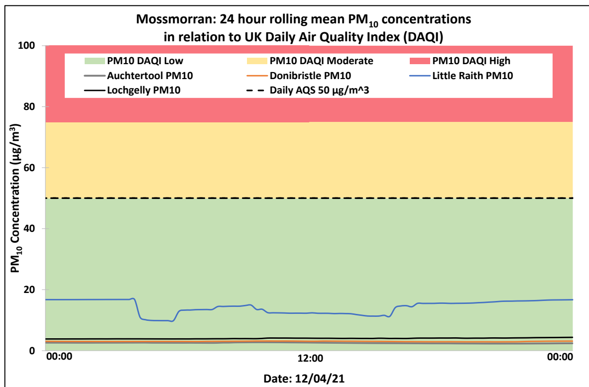
Figure 1: 24-hour rolling means for PM 10 at Lochgelly, Auchtertool, Donibristle and Little Raith on the 12 of April 2021.
