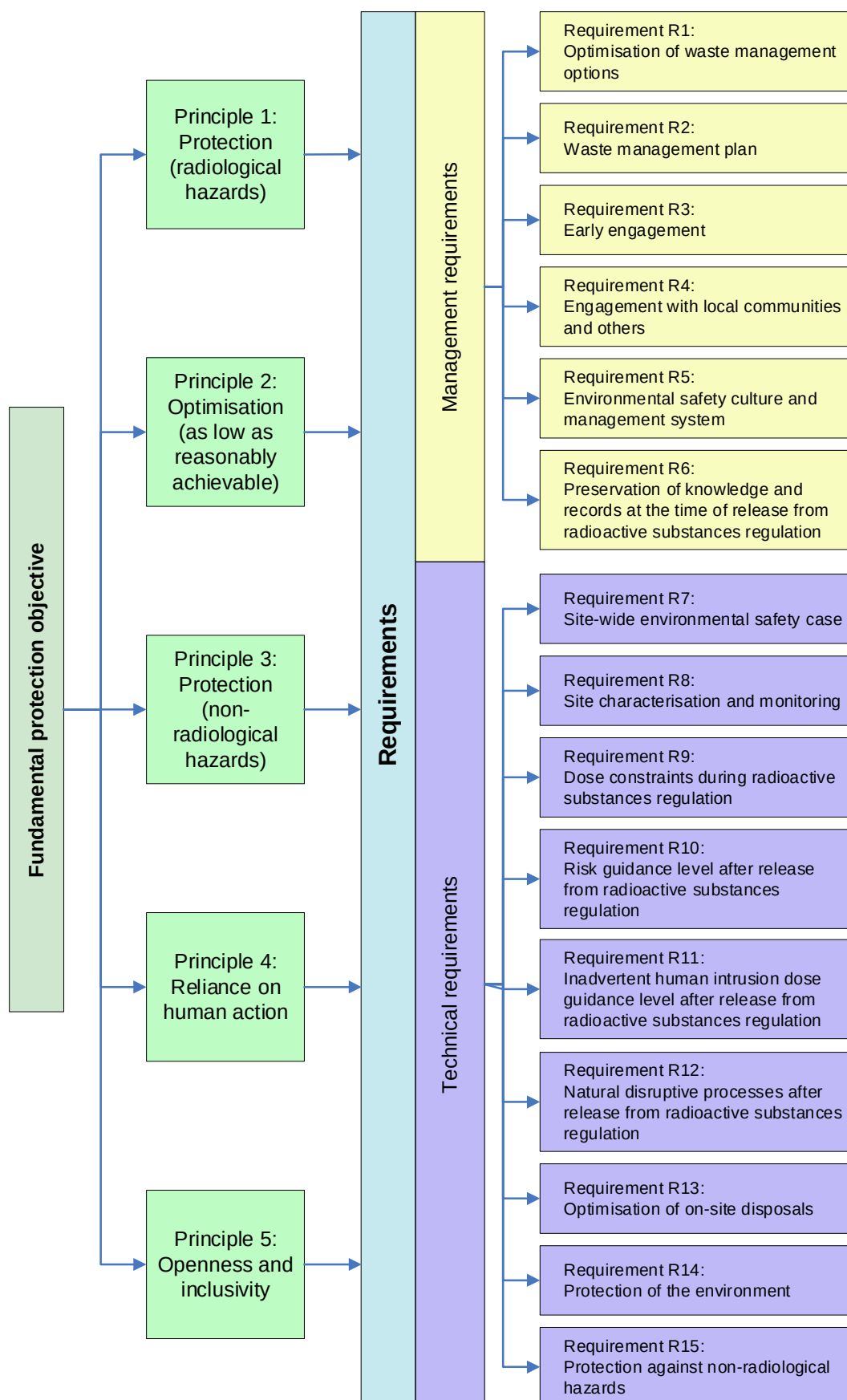
Figure 2: Relationship between protection objective principles and requirements
