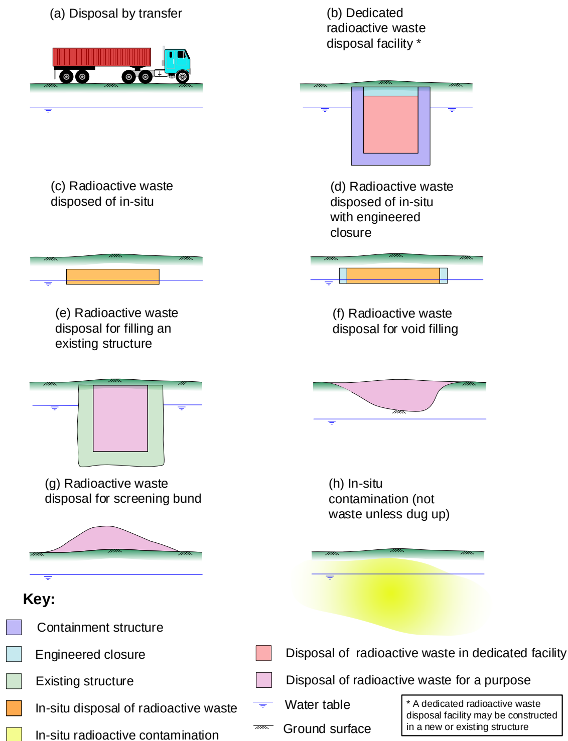
Figure 5 Potential management options for radioactive substances from the final stages of decommissioning of nuclear sites
